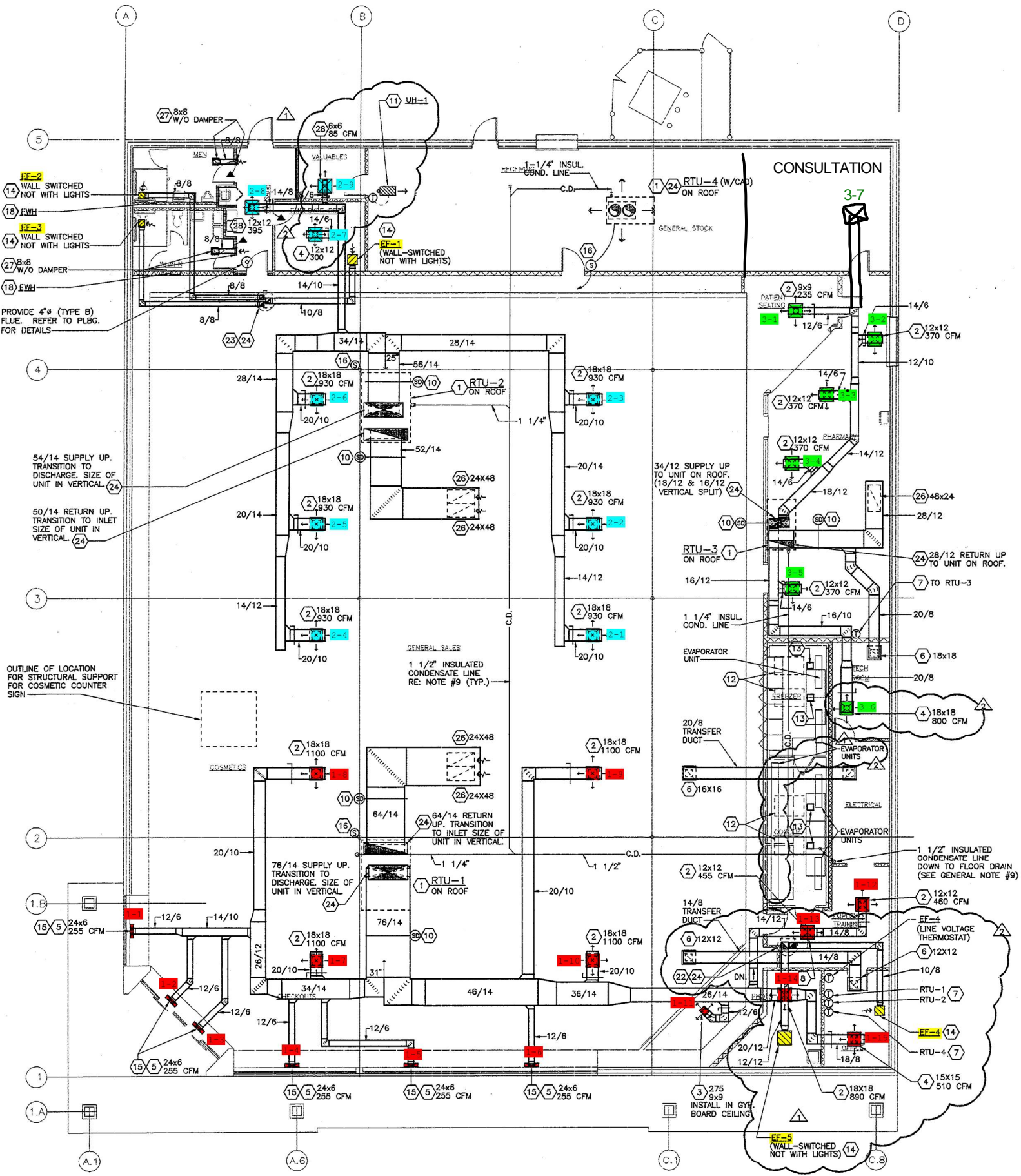
1 FLOOR PLAN - MECHANICAL SCALE: 1/8" = 1'-0"
